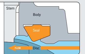
DISC OPEN 5° - 90°
